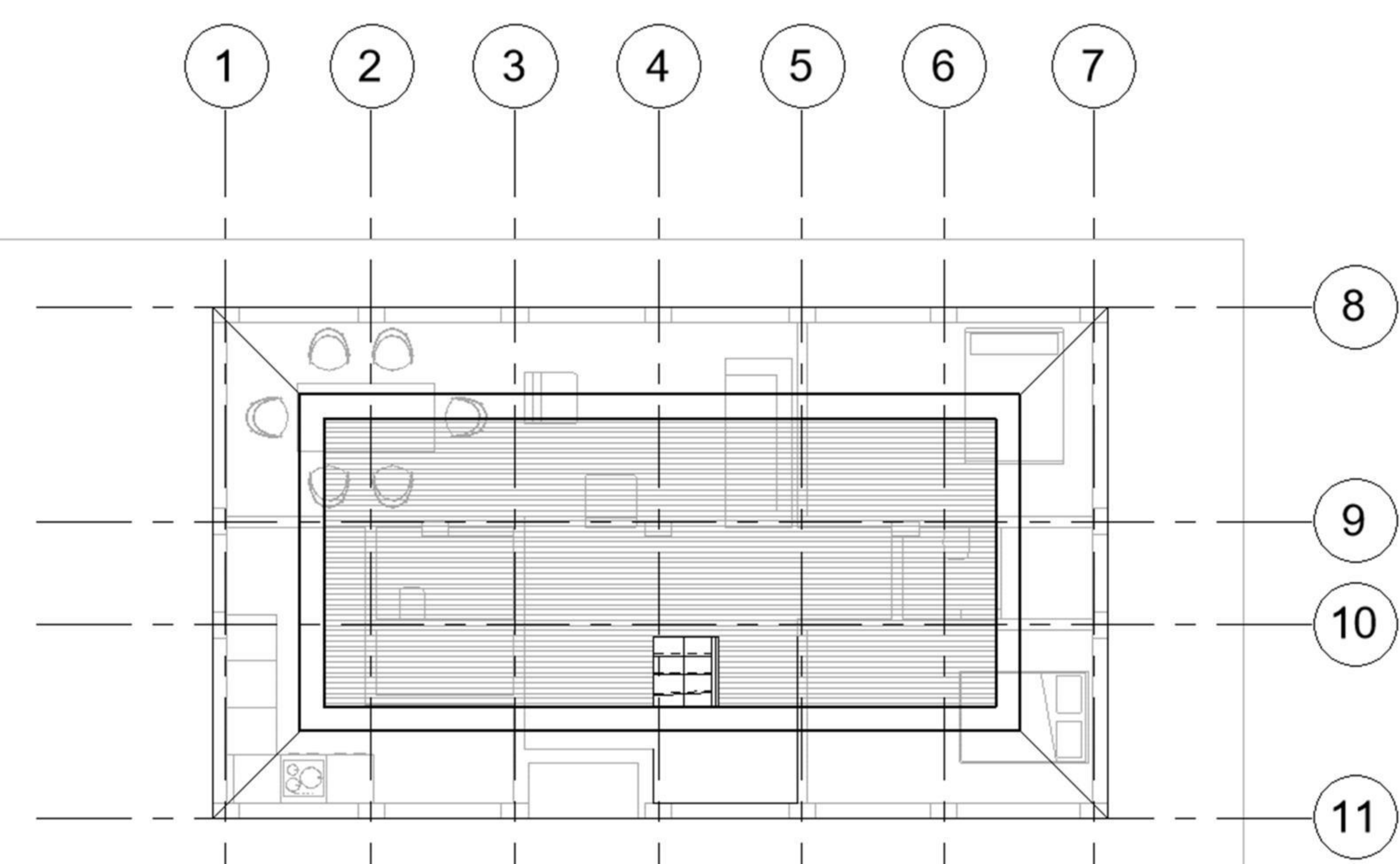
FIRST FLOR +3.50
